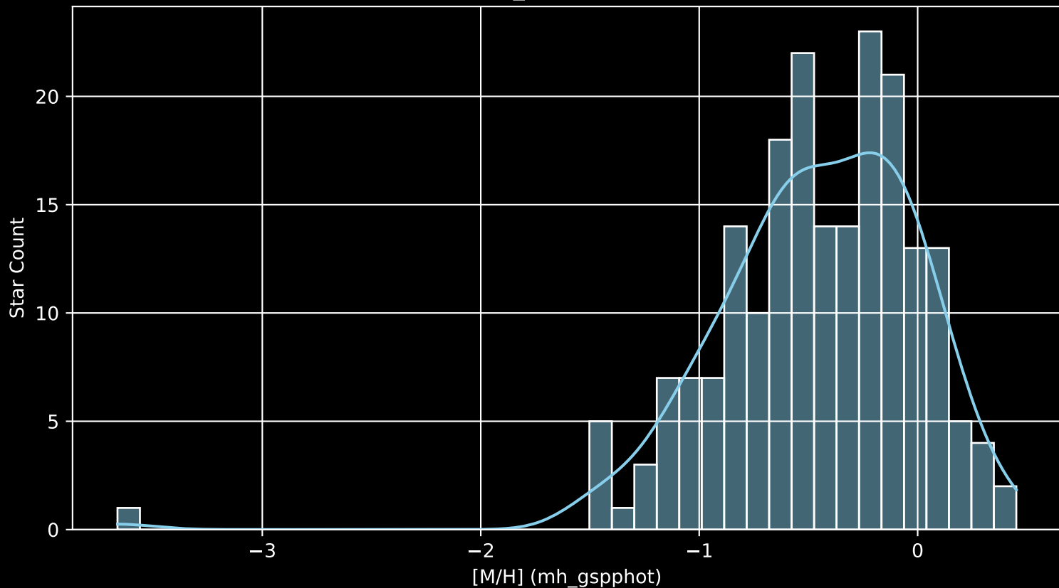
APOGEE DR17 Field: [K2_C13_175-10_btx [M/H] (mh_gspphot) (n= 204)
