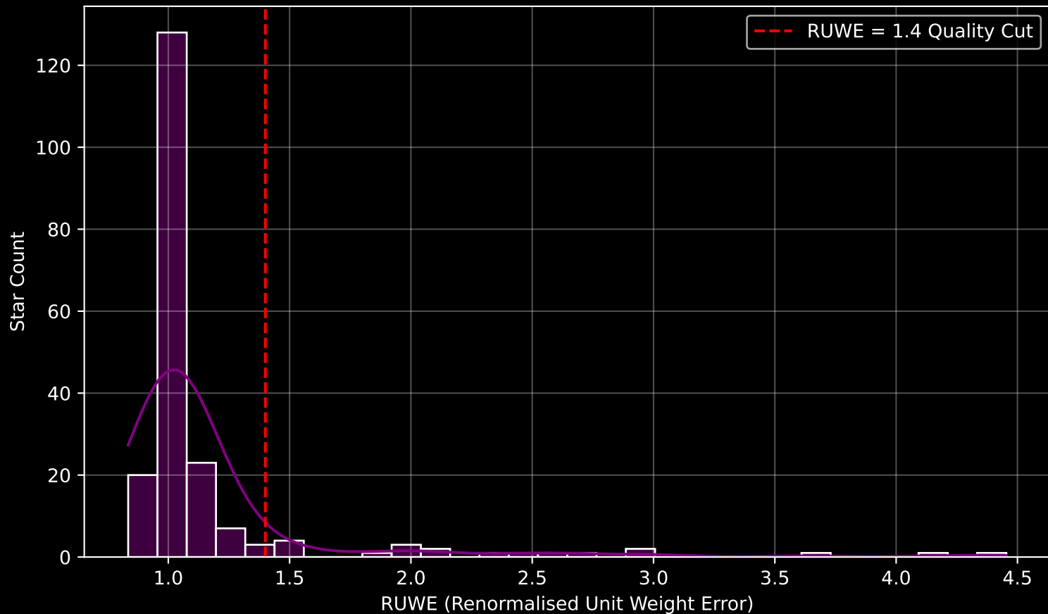
GAPOGEE DR17 Field [K2_C13_175-10_btx] RUWE Distribution (n= 200)
