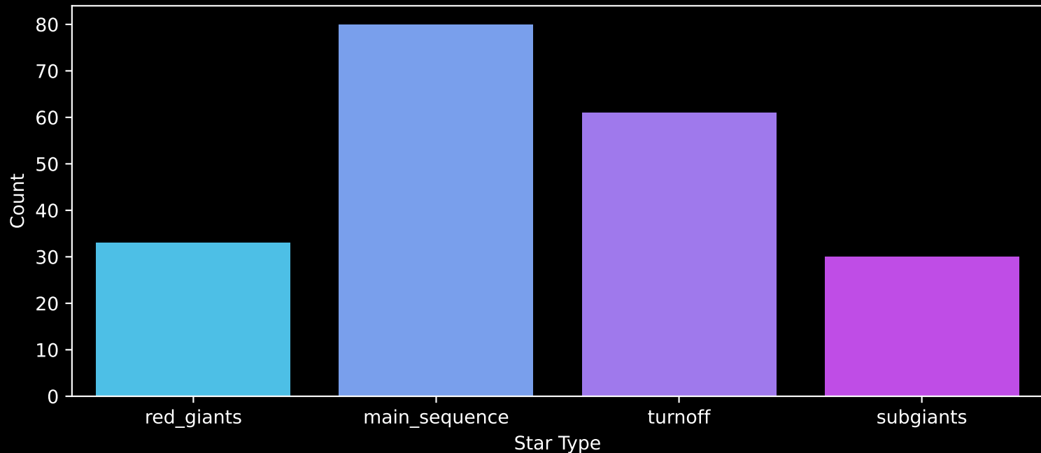
APOGEE DR17 Field: [K2_C13_175-10_btx] Count plot of Star Type
