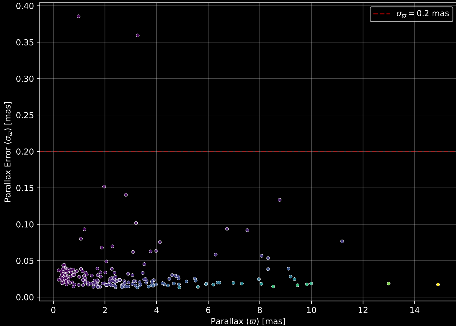
APOGEE DR17 Field: [K2_C13_175-10_btx] Parallax Quality (n= 204)
