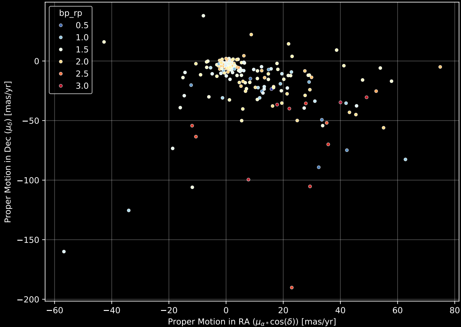
APOGEE DR17 Field: [K2_C13_175-10_btx] Proper Motion Diagram (n= 204)
