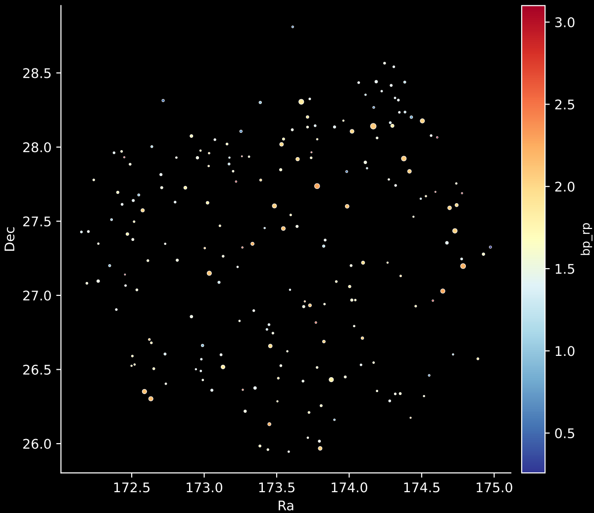
APOGEE DR17 Field: [K2_C13_175-10_btx] Stars: 204
